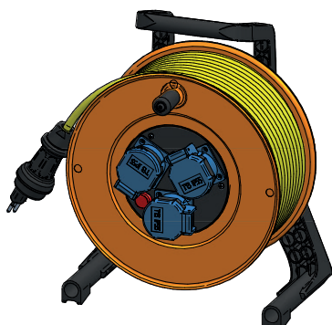
Cable reel plastic type 510 L×W×H= 297×367×208 mm
